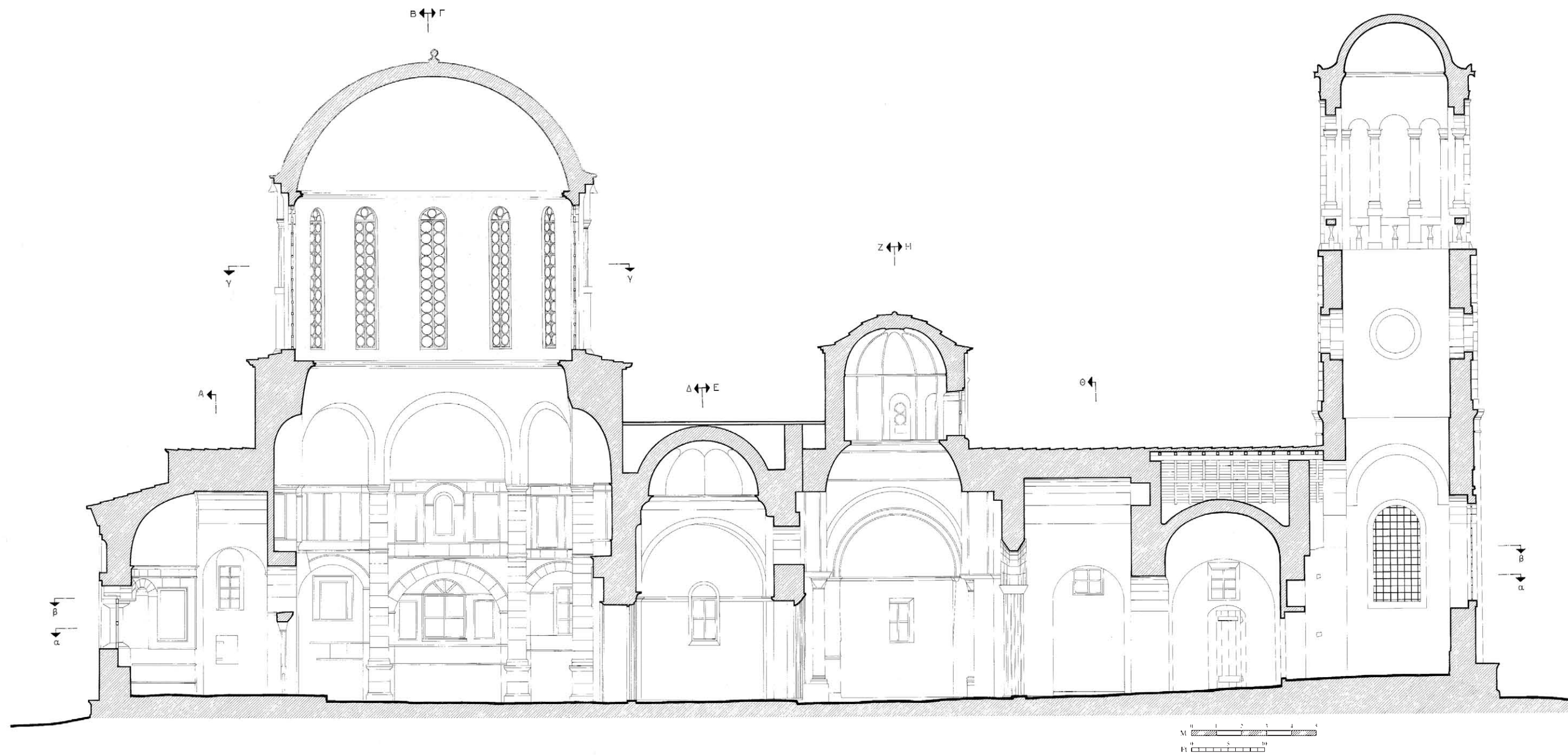
Plan 2: Katholikon, longitudinal section
