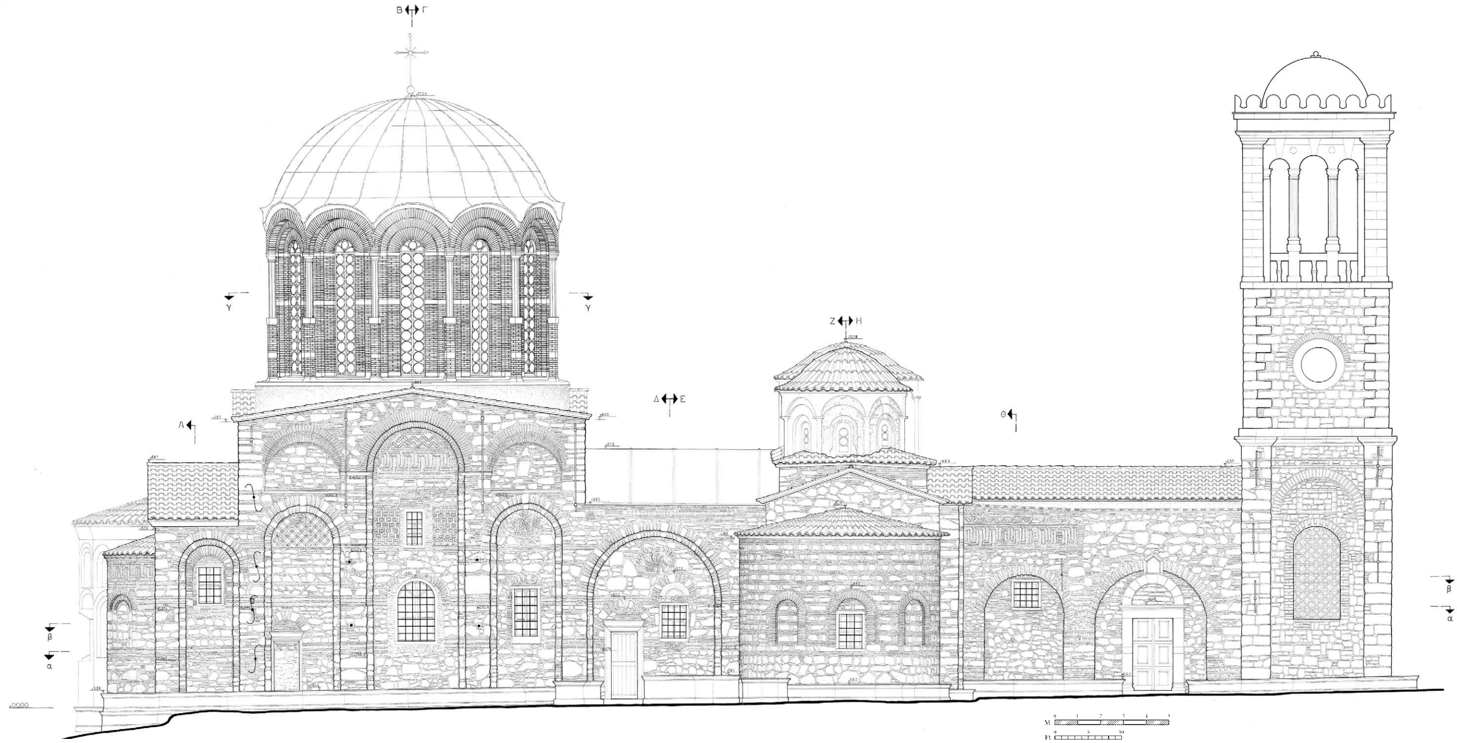
Plan 3: Katholikon, north façade.
