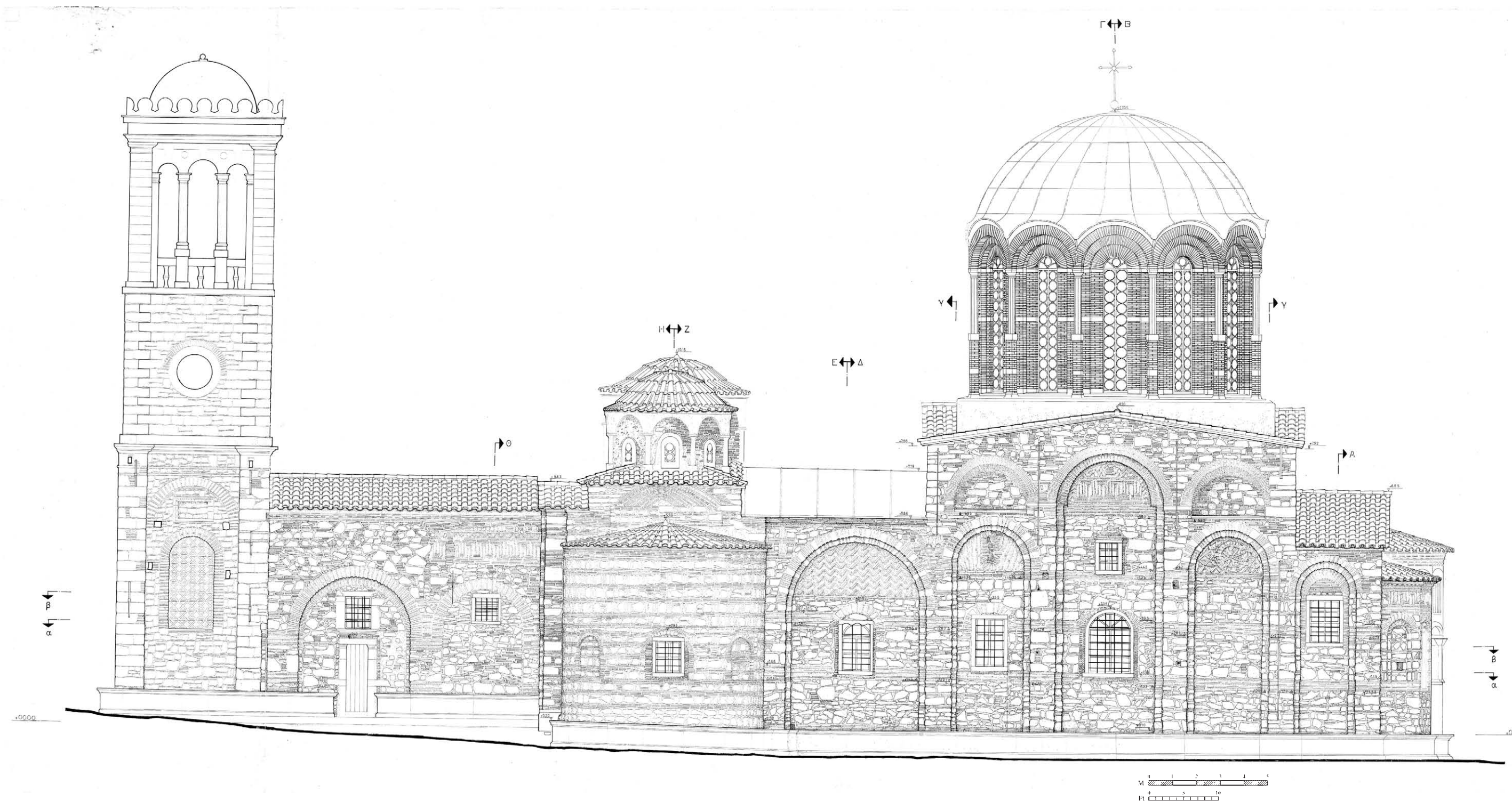
Plan 4: Katholikon, south elevation
